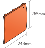
Tile-and-a-half
