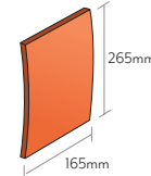
Creasing tiles
